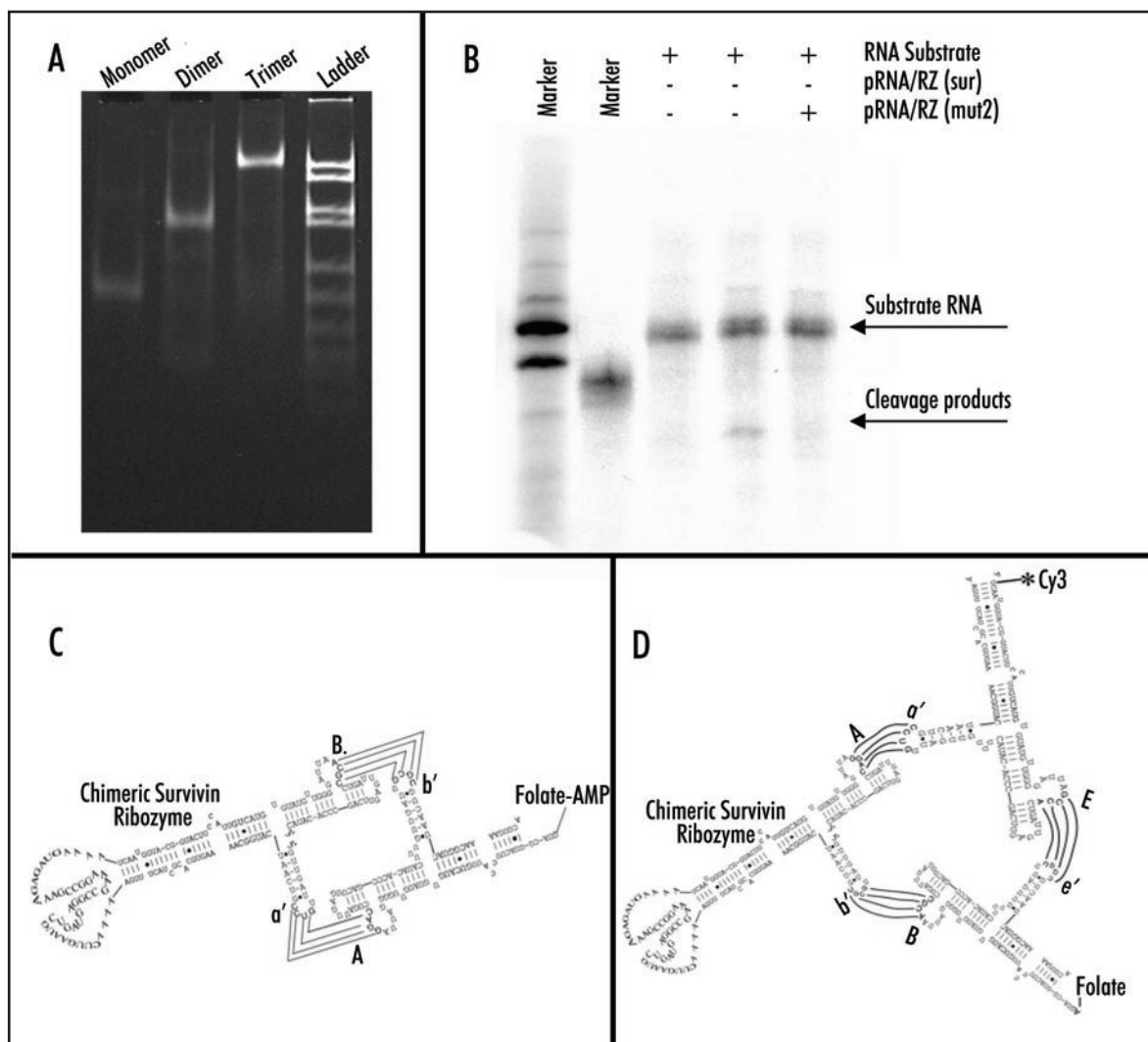
Figure 5. (A) Dimer and trimer formation of pRNA/RZ(sur) as shown in 8% native PAGE. (B) The cleavage of partial sequence of survivin mRNA by pRNA/RZ(sur). The substrate RNA is partial sequence of mRNA of human survivin labeled with [^{32}\text{P}] . (C) Deliverable dimer and trimeric complex. Each subunit of the dimer or trimer complex will be used to carry different functional motifs such as ribozyme and cell-surface recognizing aptamer or folate. In the trimeric complex, folate is used to target the folate receptor on cancer cell surface and trigger receptor mediated endocytosis. pRNA subunit with Cy3 labeling can be used to locate the complex.
