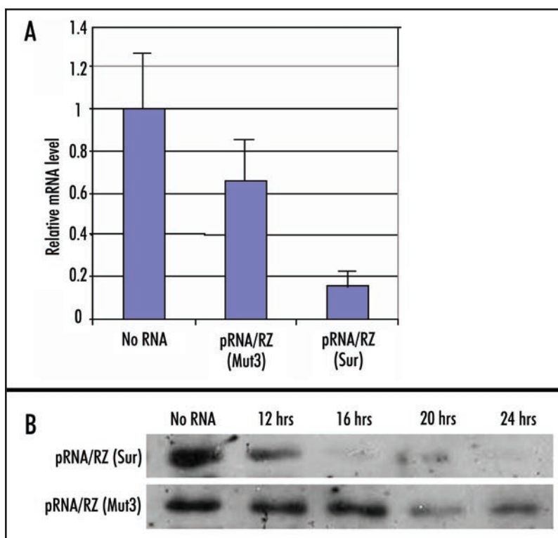
Figure 4. The effect of chimeric pRNA/RZ on mRNA and protein level. (A) Comparison of mRNA levels of different pRNA chimera treated samples revealed by real-time PCR. Gene expression level was compared to the level of gene expression found in non-transfected sample, arbitrarily assigned the value 1. Bars represent the fold number in gene expression over the expression level in the non-transfected samples. The mRNA level of pRNA/RZ treated cells decreased to 16% of that of the non-transfected cells, or 24% of pRNA/RZ(mut3) treated cells. (B). Comparison of survivin protein level by Western blot after cells were transfected with chimeric pRNA/RZ(sur) or mutant chimeric ribozyme.
