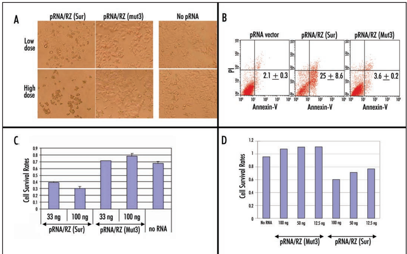
Figure 2. The effects of chimeric survivin ribozyme on breast cancer cells. (A) Cell morphology of MCF-7 after treatment of pRNA/RZ(Sur) chimera. MCF-7 were transfected with pRNA/RZ(Sur), pRNA/RZ(mut3) at high and low doses. One day after transfection, images were taken using an inverse microscope. (B). PI/annexin V double-staining to differentiate apoptosis from necrosis. Breast cancer MCF-7 cells were transfected with pRNA/RZ(sur) and apoptosis was monitored using PI/annexin V double-labeling followed by flow cytometry. Three parallel experiments were performed and the percentage of apoptotic cells was shown with standard deviation. The effects of chimeric survivin ribozyme on other breast cancer cell lines. (C). MDA-MB-231 and (D). MDA-MB-453 cells were transfected with indicated amount of RNA and cell viability was measured in the next day.
