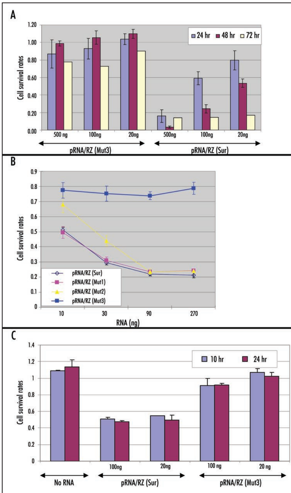
Figure 3. The effects of chimeric survivin ribozyme on (A) cervix cancer cells, (B) nasopharyngeal cancer cells and (C) prostate cancer cells. Human cervix, nasopharyngeal or prostate cancer cells were transfected with pRNA/RZ(sur) with indicated amount. Cell viability was measured by MTT assay in the next day or as indicated.
