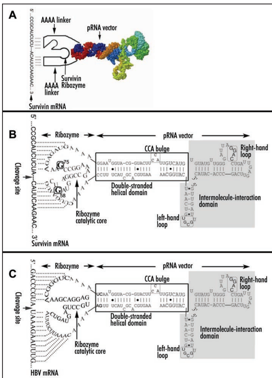
Figure 1. Sketch of sequence and structure of pRNA chimera. (A) Sketch of chimeric ribozyme harbored in pRNA vector. (B) Sequence and secondary structure of pRNA/RZ(Sur) and two cleavage disabling mutants. Both pRNA/RZ(mut1) and pRNA/RZ(mut2) have the identical pRNA vector sequence, while the sequence of catalytic core are altered. The highlighted G75 is deleted in pRNA/RZ(mut1). G75 is deleted and G58 is replaced with an "A" from pRNA/RZ(mut2). (C) Sequence of pRNA/RZ(mut 3) which targets the HBV mRNA.
